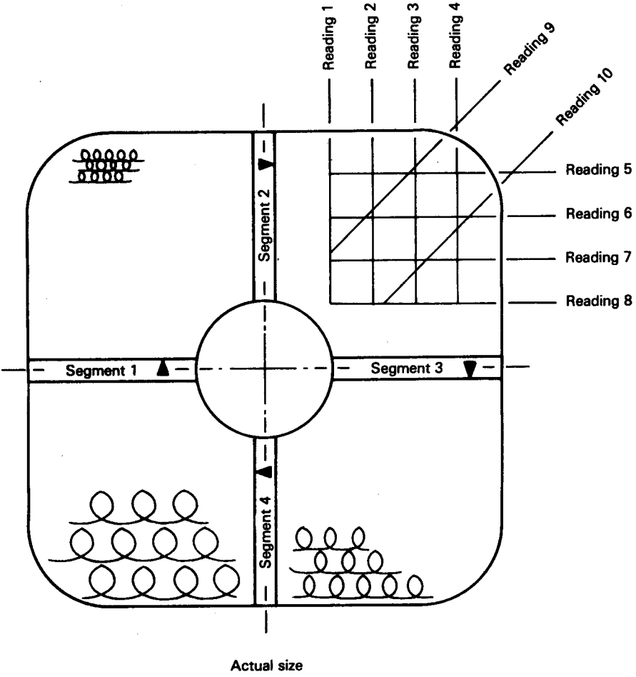
Figure 2 – Suggested traversing pattern to obtain 10 readings of R_{v5}
